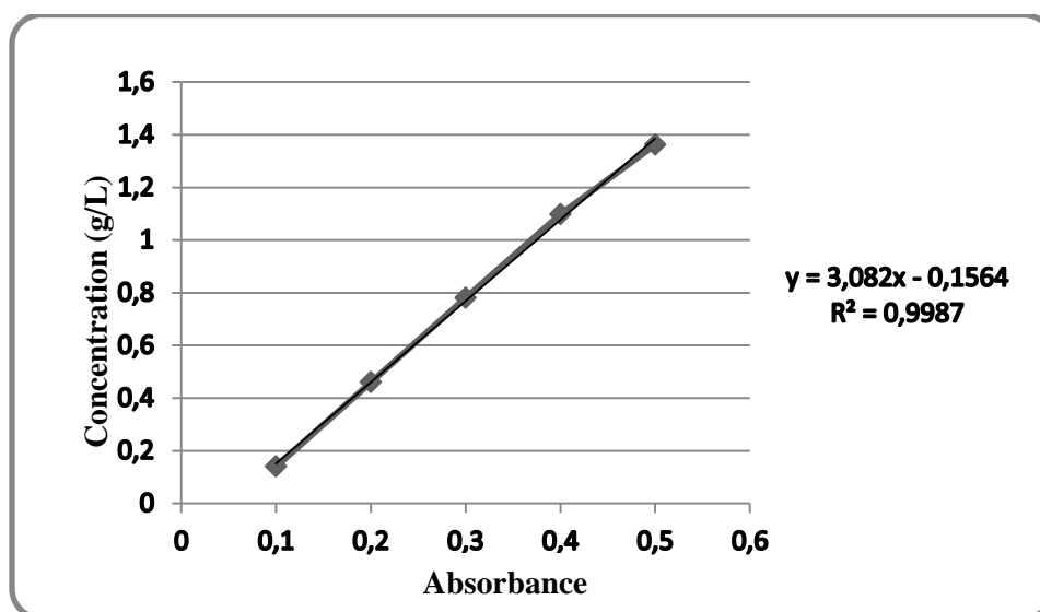
Figure 2: Standard Glucose Solution Curve
